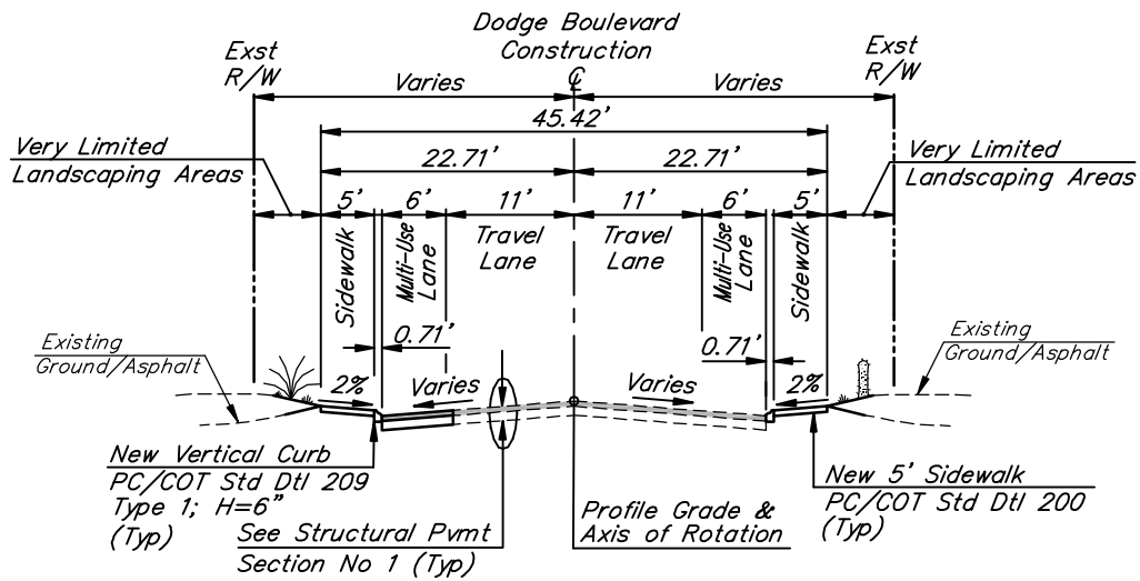
SUGGESTED TYPICAL SECTION DODGE BOULEVARD NTS
